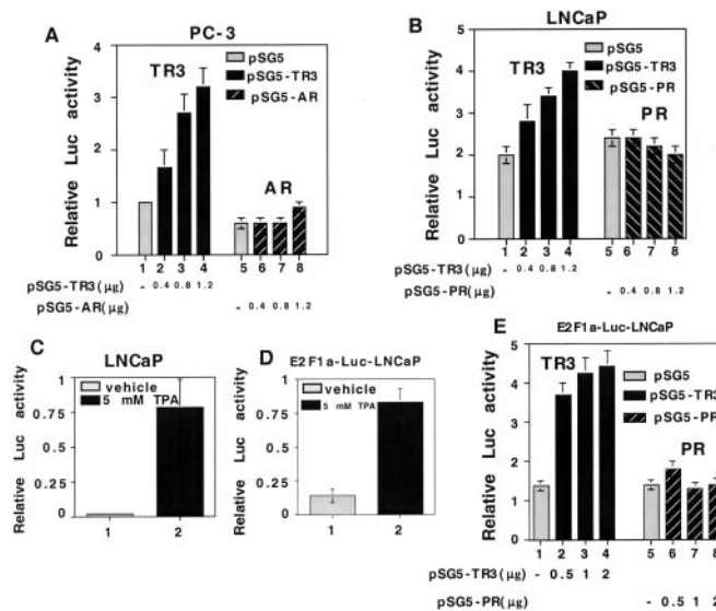
FIG. 4. Induction of E2F1 promoter activity by TR3. A and B , increasing amounts (0.4, 0.8, and 1.2 \mu\text{g} ) of pSG5-TR3 (lanes 2–4), pSG5-progesterone receptor, or pSG5-androgen receptor (lanes 6–8) were cotransfected with 0.8 \mu\text{g} of p-728E2F1-Luc (pE2F1a-Luc) reporter gene into PC-3 (A) and LNCaP (B) cells. After 16–24 h, cells were collected and assayed for Luc activity. C , pE2F1a was transfected into LNCaP cells, and the cells were treated with 5 mM TPA for 4 h. Cells were collected and assayed for Luc activity. D , E2F1a-Luc-LNCaP cells were treated with vehicle (lane 1) and 5 mM TPA (lane 2) for 4 h. Cells were collected and assayed for Luc activity. E , increasing amounts (0.5, 1, and 2 \mu\text{g} ) of pSG5-TR3 (lanes 2–4) and pSG5-progesterone receptor (lanes 6–8) were transfected into E2F1a-Luc-LNCaP cells. After 16–24 h, cells were collected and assayed for Luc activity. The results in Fig. 4 were normalized with either pRLSV40-Luc (A and B) or pRL-TK (C and E) and expressed as the mean \pm S.E. of more than three independent experiments.
