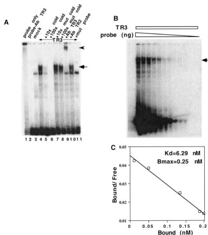
FIG. 3. The specific binding and higher binding affinity of TR3 to E2F1-TR3RE. A , binding of in vitro expressed TR3 to E2F1-TR3RE. EMSA was performed with the in vitro expressed TR3 and the ^{32}\text{P} -labeled E2F1-TR3RE oligomers (lanes 1–10) or ^{32}\text{P} -labeled mutant E2F1-TR3RE oligomer probes (lane 11). As negative controls, the binding reaction contained either no lysate (lane 1, probe only; lane 2, anti-TR3 antibody (Ab) only) or lysate without TR3 (lane 3, probe and mock translated products). Binding reaction mixtures were incubated with the probe and in vitro expressed TR3 (lanes 4–11) in the presence of 10- (lane 5) or 100-fold (lane 6) excess of unlabeled E2F1-TR3RE as competitors or 10- (lane 7) or 100-fold (lane 8) excess unlabeled mutated E2F1-TR3RE as controls. Supershift of the TR3 protein-E2F1-TR3RE complex was induced in the presence of anti-TR3 antibody (lane 9) but not by anti-TR2 antibody (lane 10). When mutant E2F1-TR3RE was used as the probe, no TR3 protein-E2F1-TR3RE complex was formed (lane 11). The position of the TR3 protein-DNA complex and the supershift band are indicated by an arrow and arrowhead, respectively. B , the binding profile of in vitro expressed TR3 to various amounts of the probe. EMSA was performed with a constant amount of TR3 and varying concentrations of the labeled E2F1-TR3RE probe (0.0039–2 ng). The binding mixtures were resolved by 5% polyacrylamide gel. C , Scatchard analysis of TR3 affinity for E2F1-TR3RE. After autoradiography, the respective bands were excised, placed in scintillation fluid, and quantified directly in a scintillation counter. The ratio of activity between specific DNA protein binding ( Bound ) and free DNA probe with respect to specific DNA protein binding ( Bound/Free ) was plotted. The dissociation constant ( K_d ) and B_{\text{max}} were determined from the minus reciprocal of the slope of the line generated from the experimental data.
