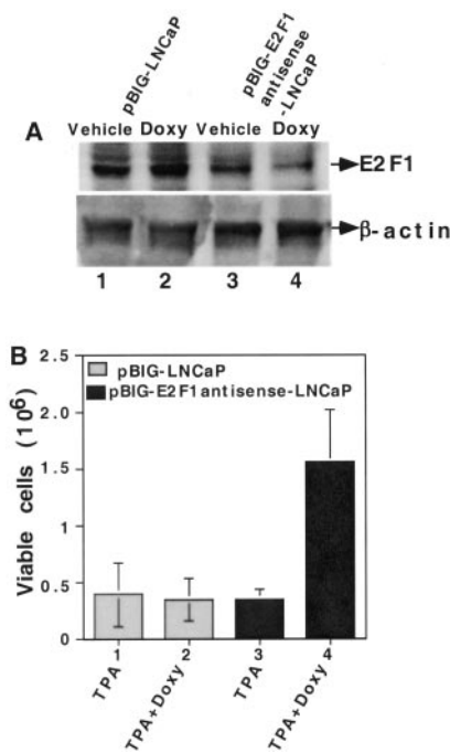
FIG. 2. Expression of antisense E2F1 can partially rescue TPA-induced cell death in pBIG-E2F1 antisense-LNCaP cells. A, the suppression of E2F1 by the treatment of 6 \mu g/ml doxycycline (Doxy) to induce E2F1 antisense expression in pBIG-E2F1 antisense-LNCaP cells is shown. pBIG-E2F1 antisense-LNCaP cells (lanes 3 and 4) and pBIG-LNCaP cells (lanes 1 and 2) were treated with 6 \mu g/ml doxycycline (lanes 2 and 4) and vehicle control (lanes 1 and 3) for 24 h. The cell lysates were collected and Western blot was performed. A representative blot from three independently performed experiments is shown. B, E2F1 antisense expression partially rescues TPA-induced cell death. pBIG-E2F1 antisense-LNCaP cells and pBIG-LNCaP cells were treated with control vehicle, 5 mM TPA, and 5 mM TPA plus 6 \mu g/ml doxycycline for 72 h, and viable cells were counted with trypan blue exclusion assay.
